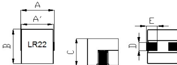
Dimension (Unit:mm):
