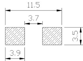
Recommended Land Pattern (Unit:mm):
