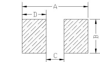
Recommended Land Pattern (Unit:mm):
